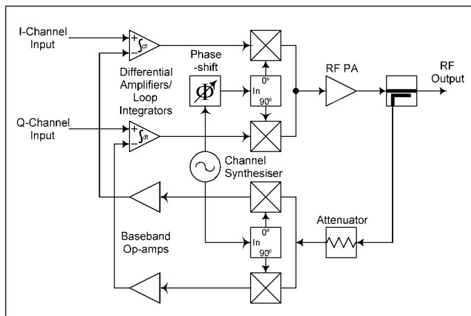
Figure 44 · Cartesian-loop transmitter configuration.
