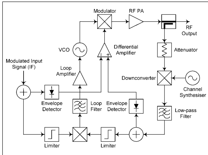
Figure 43 · Block diagram of a polar-loop transmitter.
