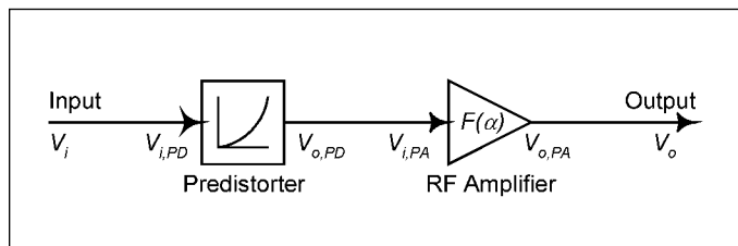
Figure 49 · Predistortion concept.
