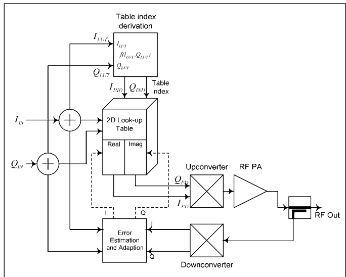
Figure 53 - Mapping predistorter.
